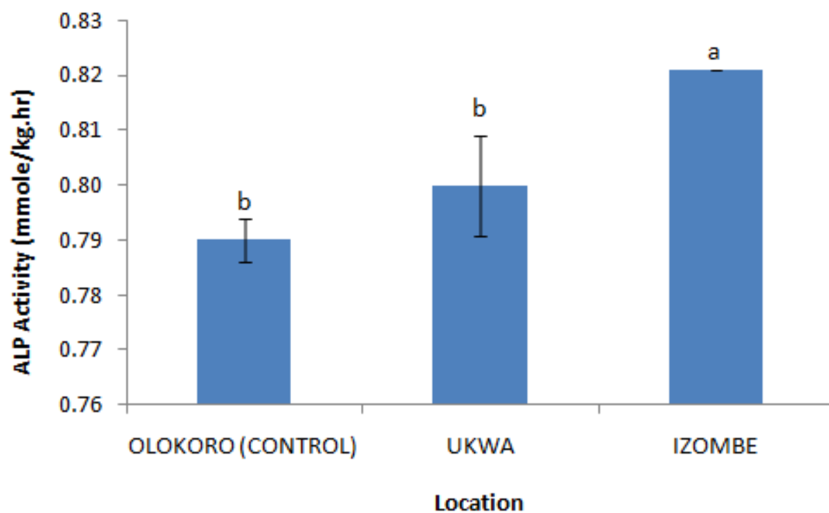
Figure 5: Effect of gas flaring on alkaline phosphatase (ALP) activity in soils from test sites
