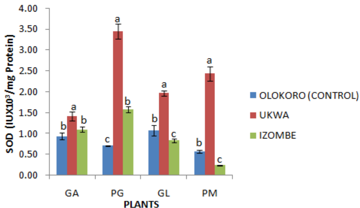
Figure 6: Effect of gas flaring on plant superoxide dismutase (SOD) activity
