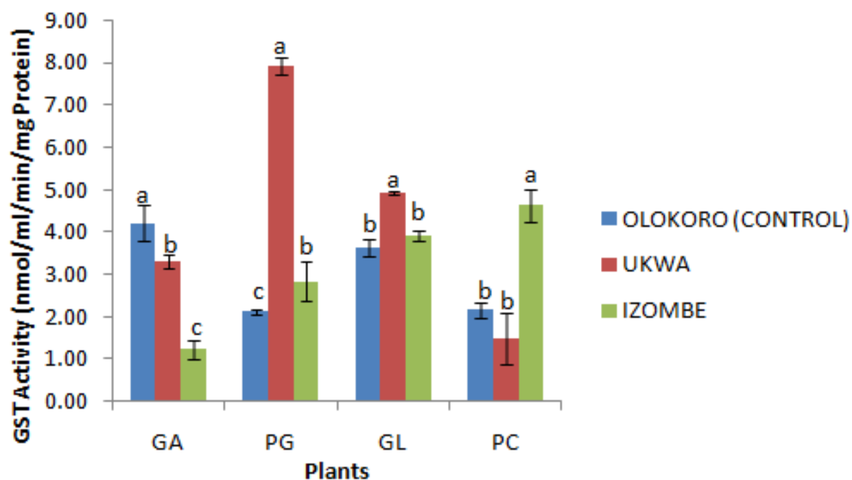
Figure 8: Effect of gas flaring on GST activity from plant leaves of test sites
