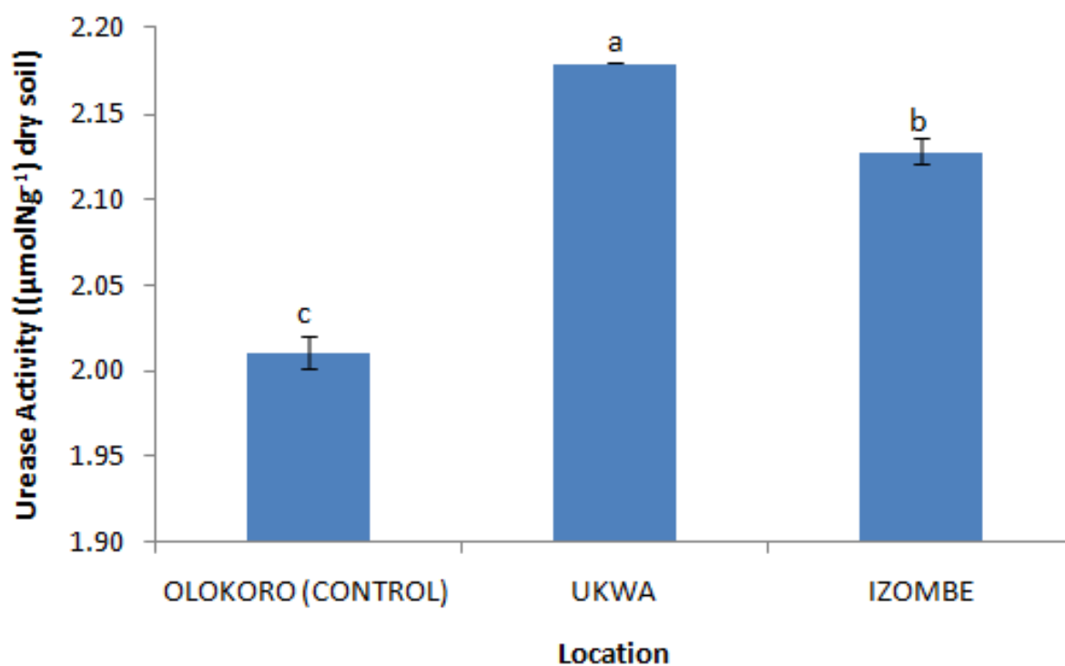
Figure 2: Effect of gas flaring on urease activity in soils from test sites.
