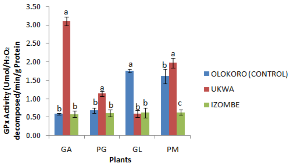
Figure 9: Effect of gas flaring on glutathione peroxidase (GPx) activity from plant leaves of test sites
