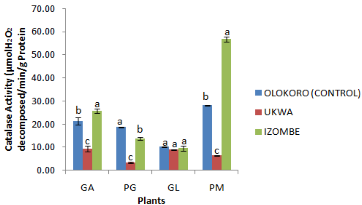
Figure 7: Effect of gas flaring on catalase activity of plant leaves from test sites
