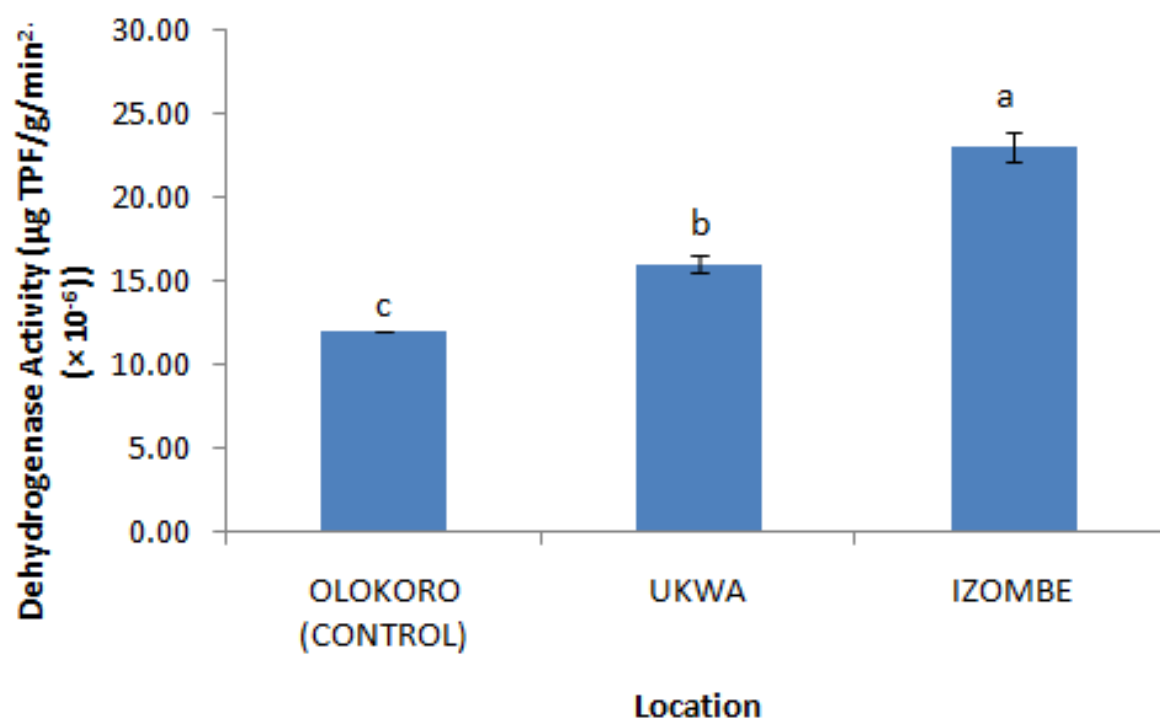
Figure 3: Effect of gas flaring on dehydrogenase (DHA) activity in soils from test sites
