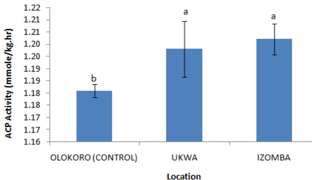
Figure 4: Effect of gas flaring on acid phosphatase (ACP) activity in soils from test sites
