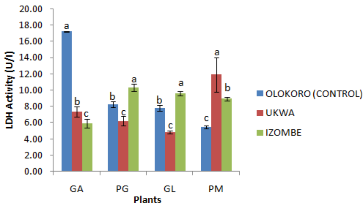
Figure 10: Effect of gas flaring on lactate dehydrogenase (LDH) activity from plant leaves of test sites
